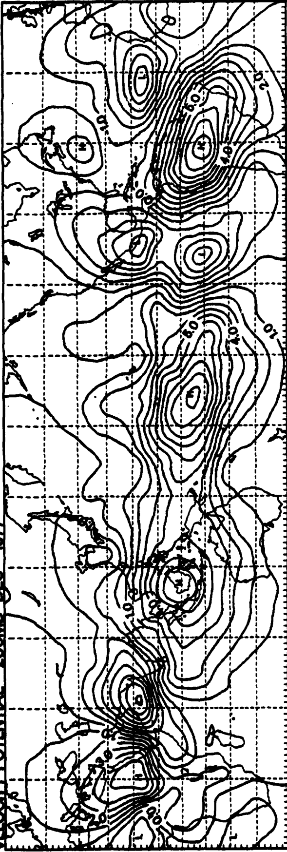
VELOCITY POTENTIAL 200MB DEC 1977
